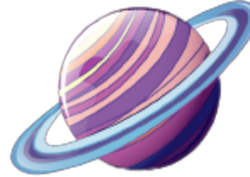
Saturn
